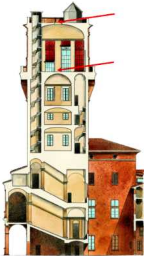
Fig. 5. Section of the Specola tower in Bologna. The lower arrow indicates the expected position of the prototype of the tessellated mirror; the higher arrow indicates the focal plane of the instrument.
